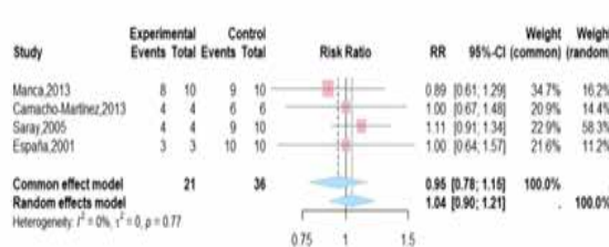
Fig. 4 Subgroup analysis
